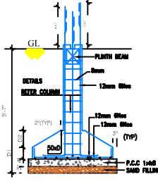
FOUNDATION DETAILS
