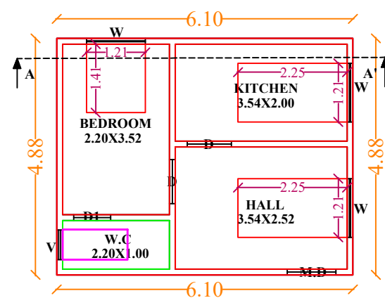
PRO GROUND FLOOR
