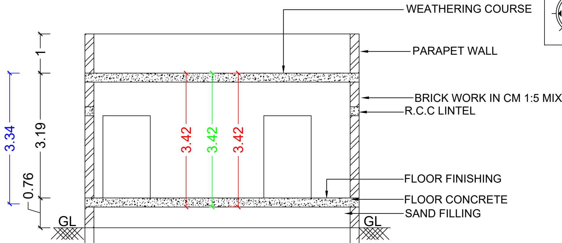
SECTION AT A1-A1
