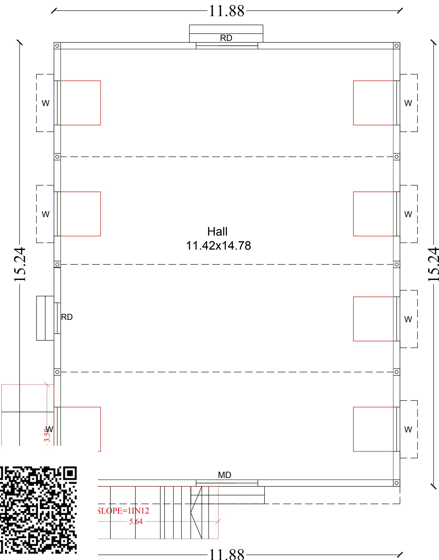
Plan
