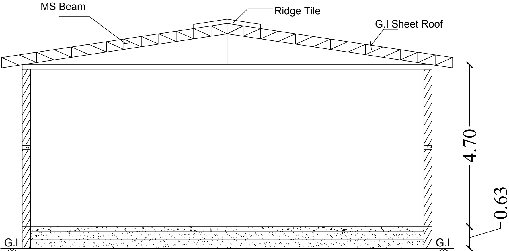
Section on-"AA"
