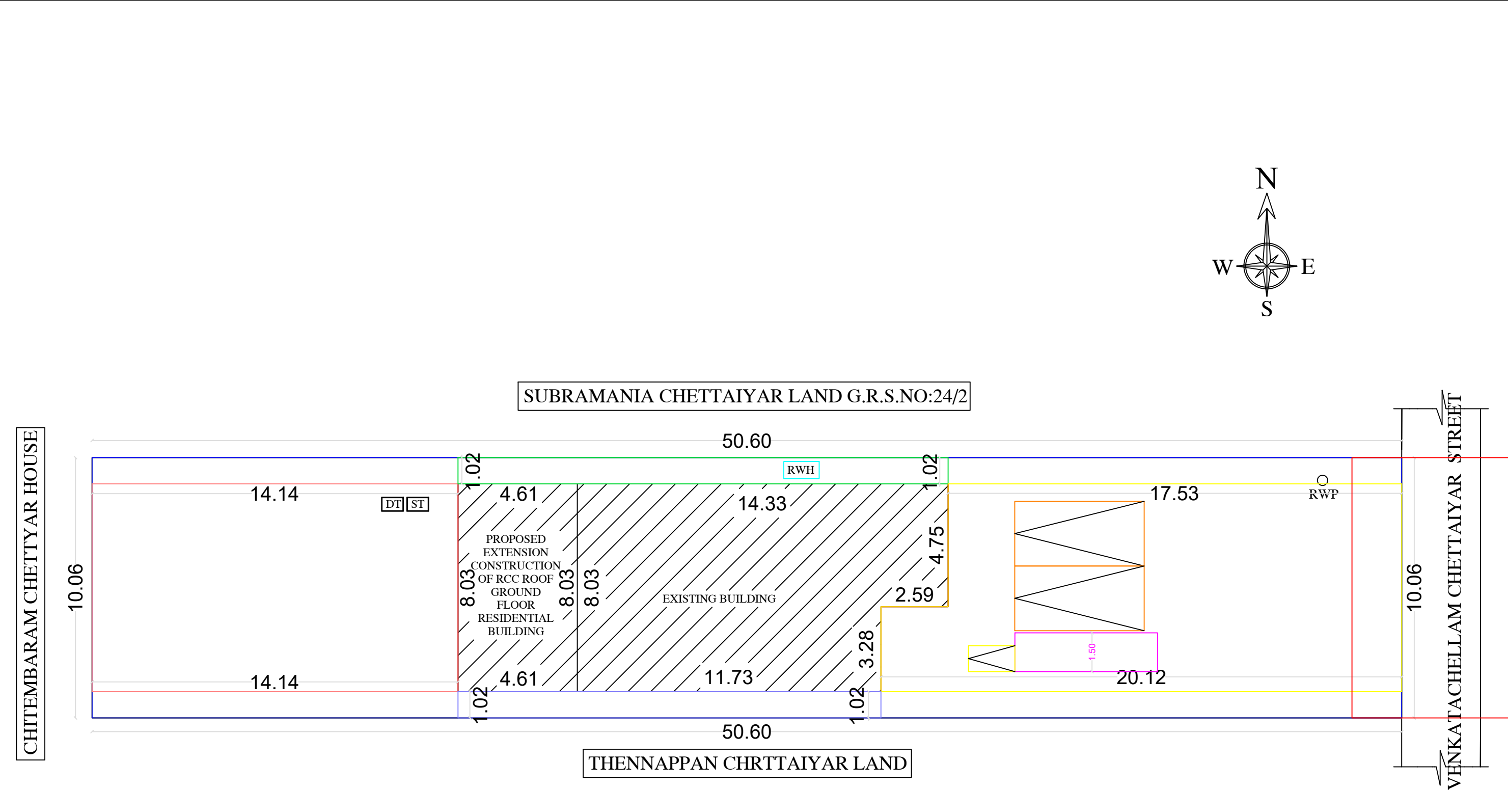
SITE PLAN
