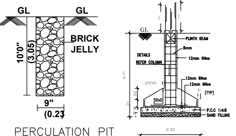
FOUNDATION DETAILS SCALE : 1:50.
