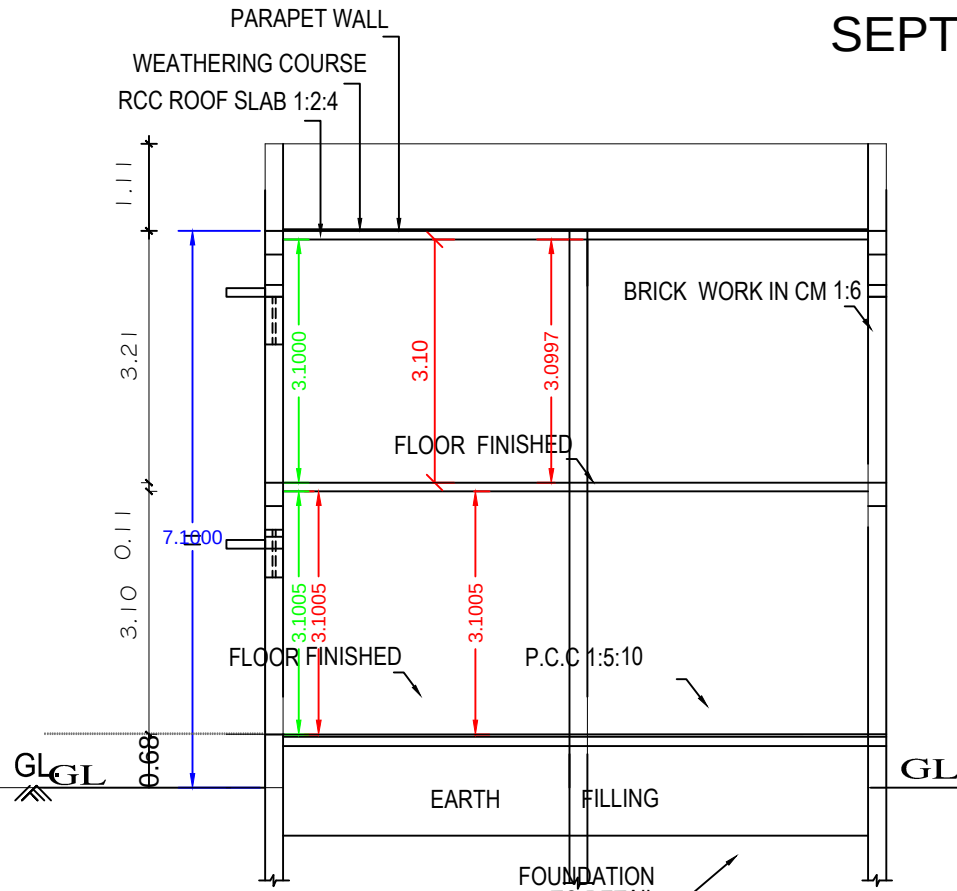
SECTION "A-B"
