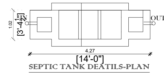
SEPTIC TANK DETAILS-PLAN
