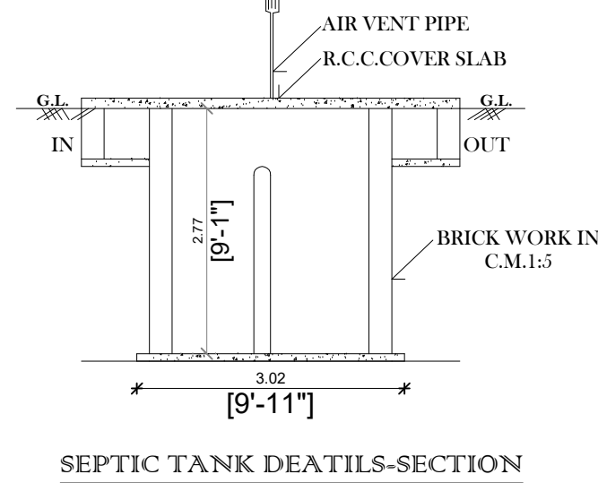
SEPTIC TANK DETAILS-SECTION
