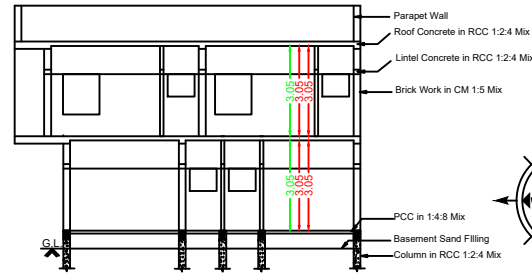
Section RR
