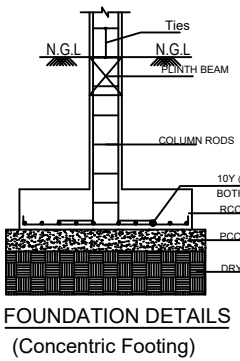
FOUNDATION DETAILS
