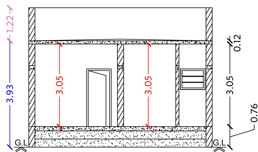
Section on-"AA"
