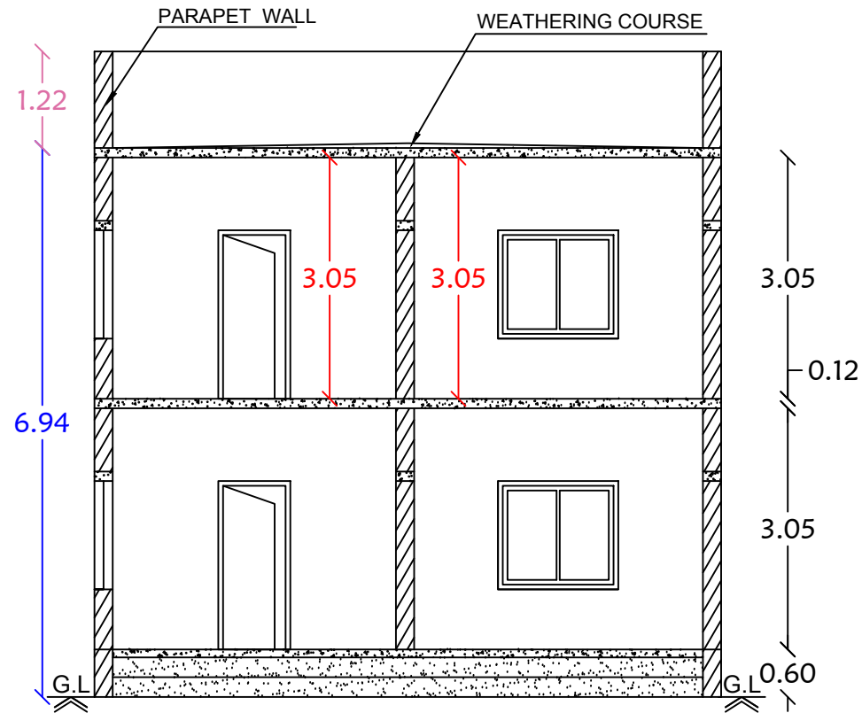
Section on-"AA"
