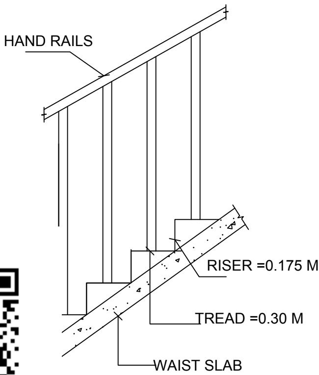
CASE DETAILS
