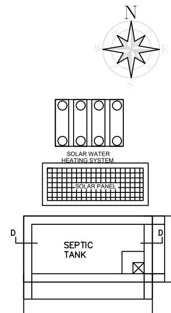
PLAN OF SEPTIC TANK SCALE 1"=2'0"
