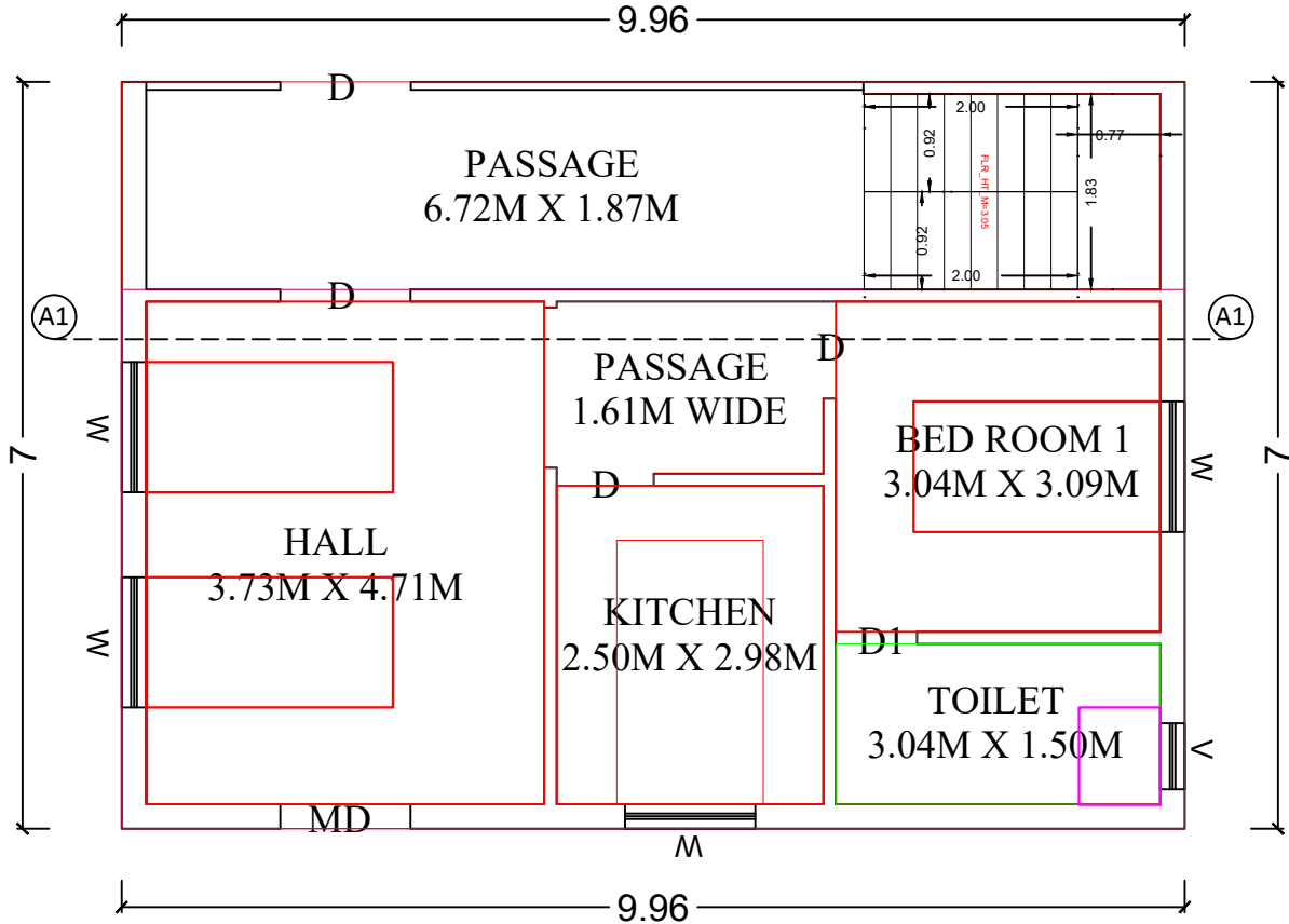
GROUND FLOOR PLAN (PROPOSED)
