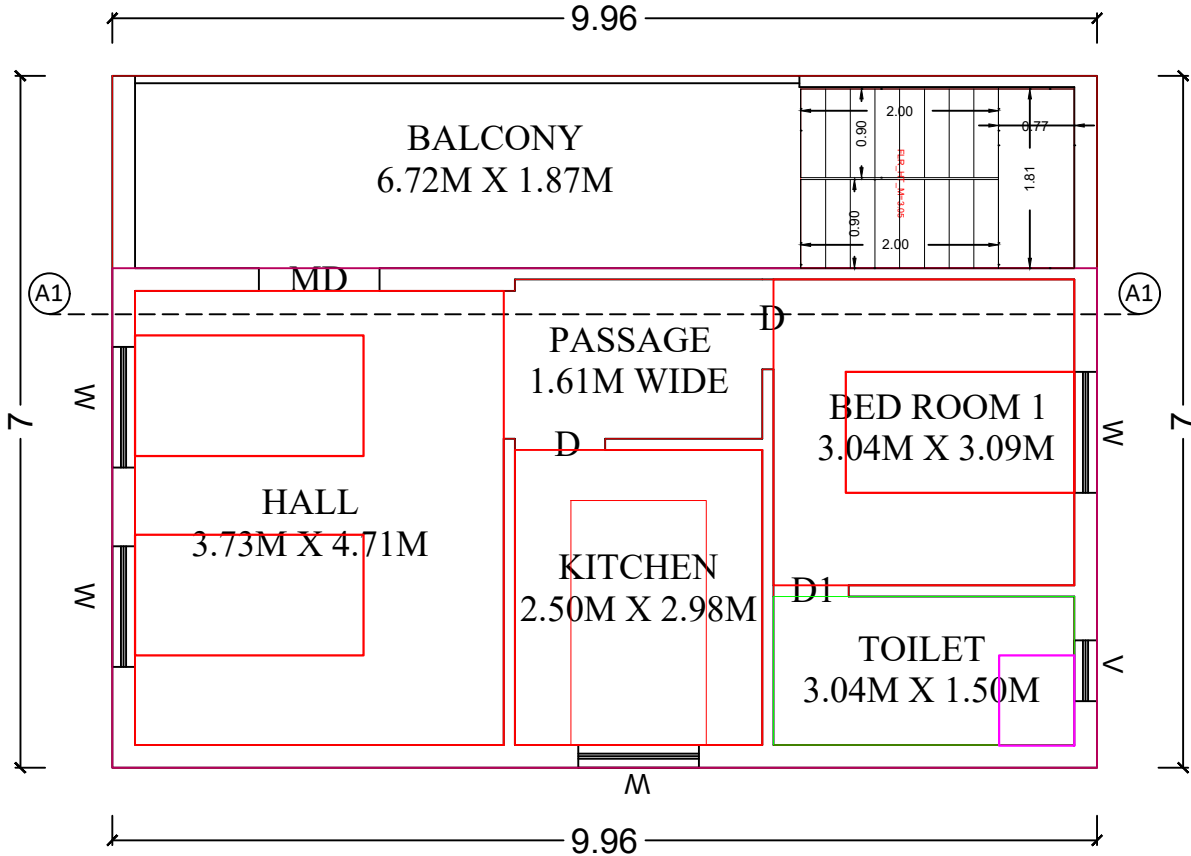
FIRST FLOOR PLAN (PROPOSED)
