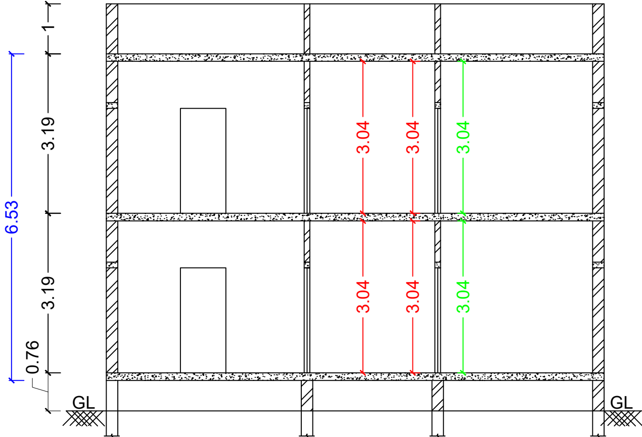
SECTION AT A1-A1
