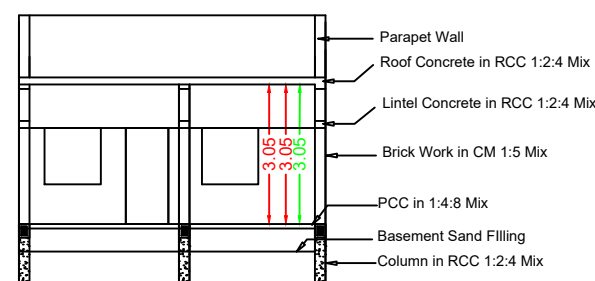
Section RR
