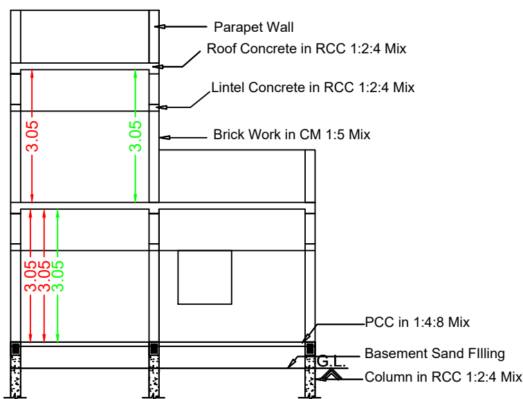
Section RR
