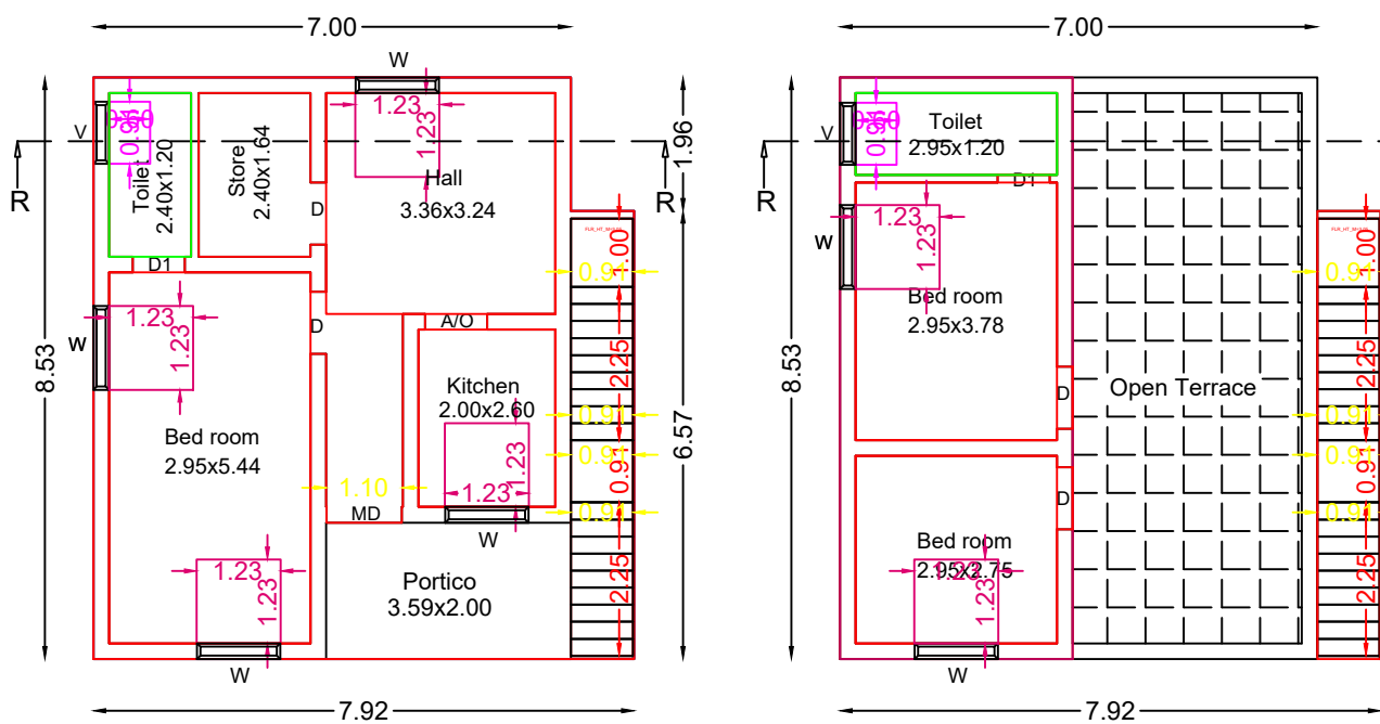
Pro.Ground & First Floor Plan
