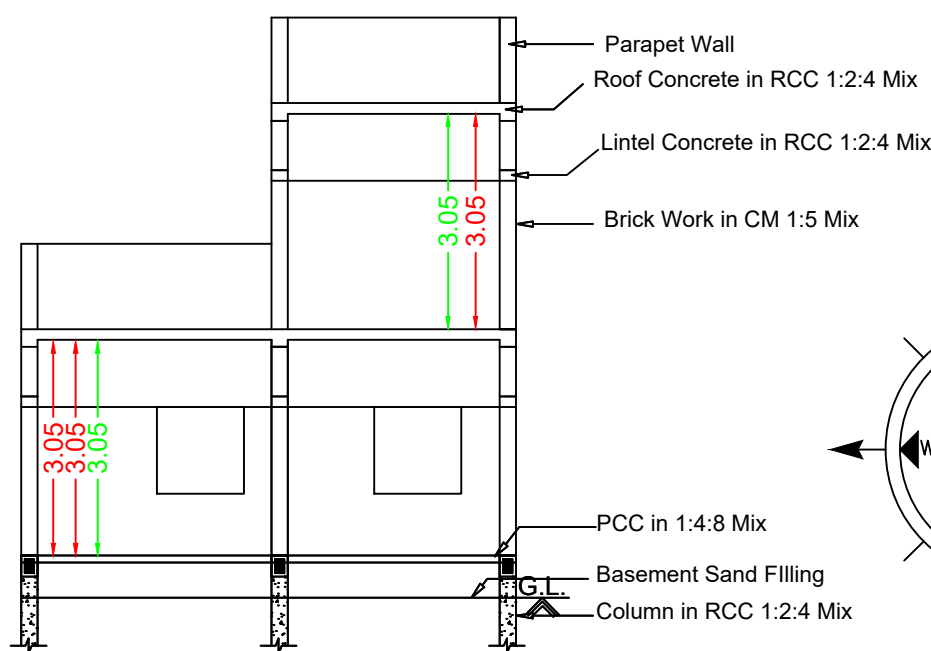
Section RR
