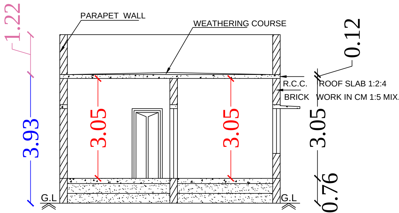
Section on-"AA"
