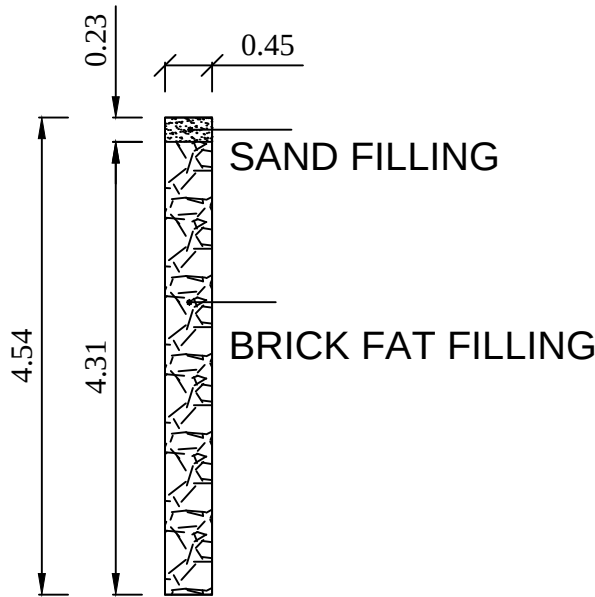
DETAILS OF PERCOLATION PIT
