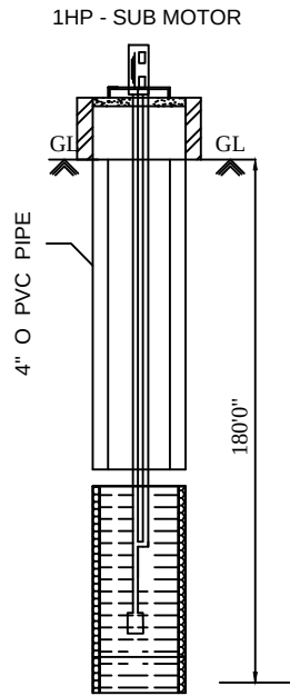
Bore Well Details
