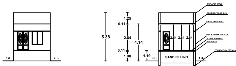
FRONT ELEVATION
