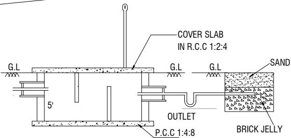
SECTION-AB
