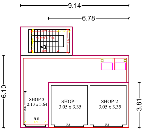
EX & PRO.GROUND FLOOR PLAN
