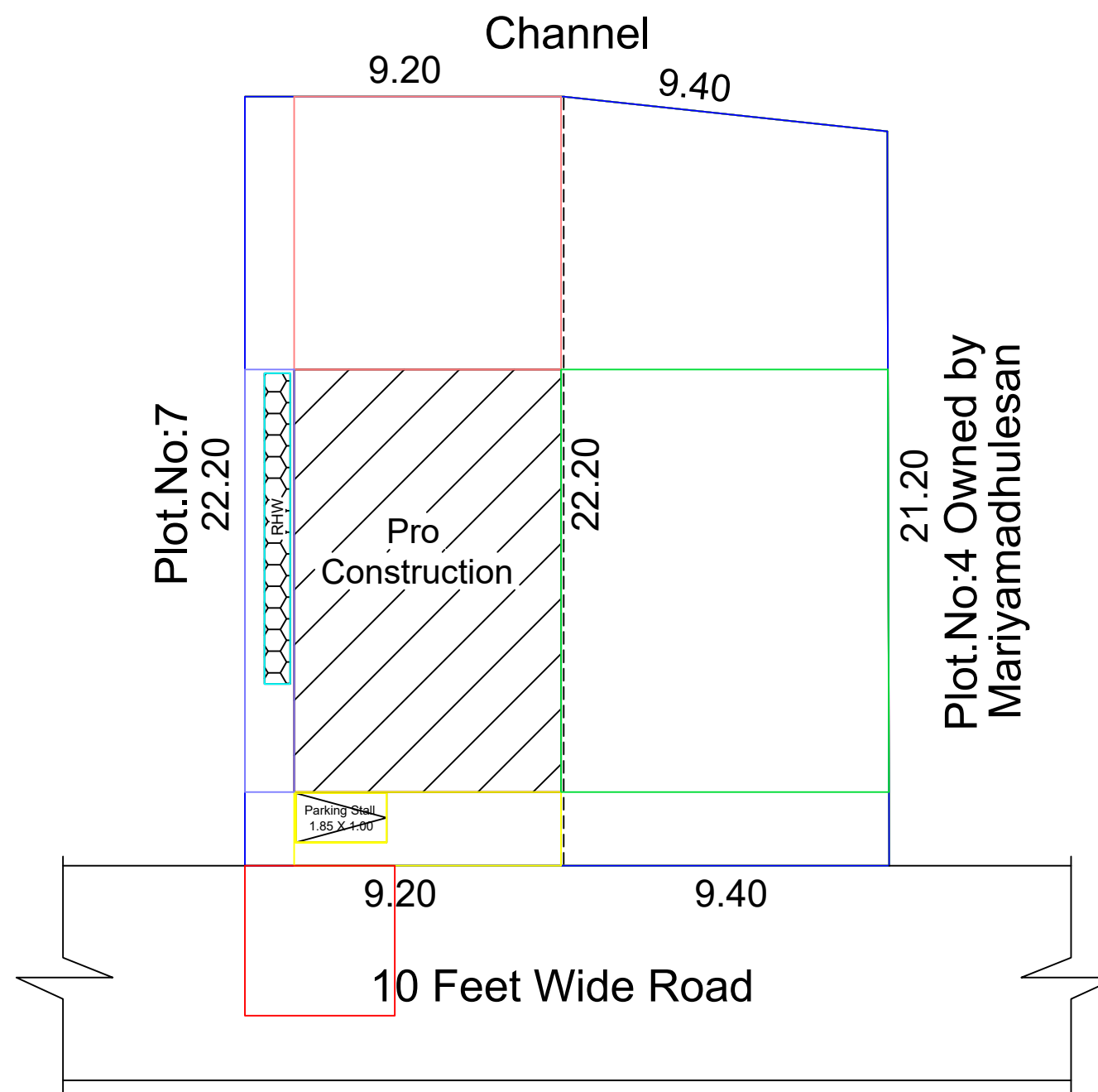
Site Plan
