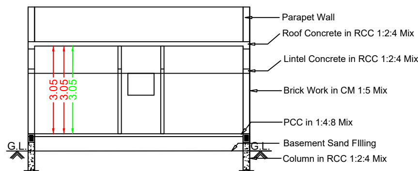
Section RR
