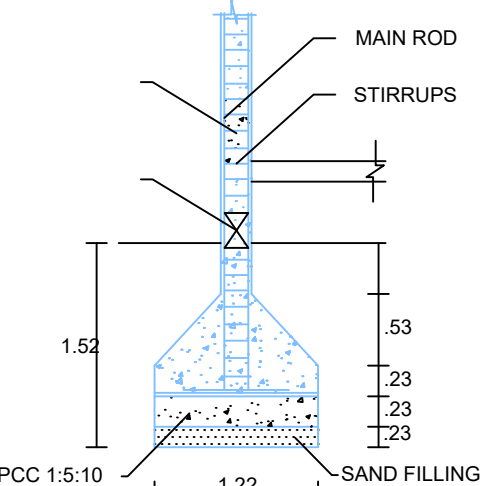
COLUMN DETAILS
