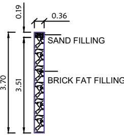
DETAILS OF PERCOLATION PIT
