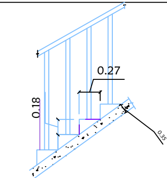
SECTION OF STAIRCASE
