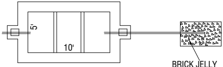
SEPTIC TANK & DISPERSION TRENCH DETAILS
