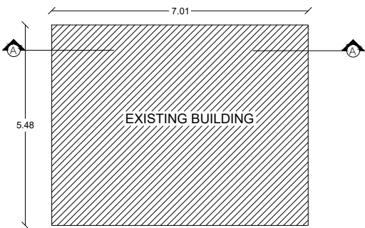
EXTGROUND FLOOR
