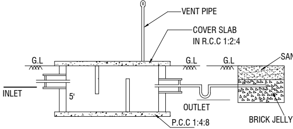
SECTION-AB
