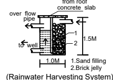
(Rainwater Harvesting System)
