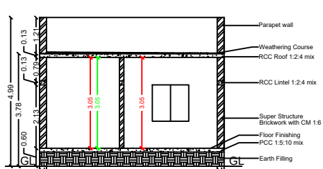
SECTION ON "VR"
