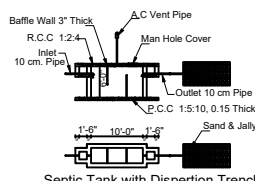
Septic Tank with Dispersion Trench
