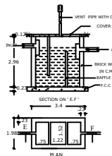
SEPTIC TANK DETAILS ( NOT TO SCALE )
