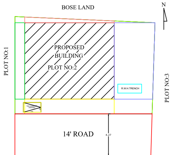
Site Plan
