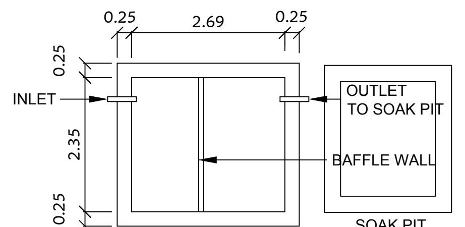
PLAN SEPTIC. TANK
