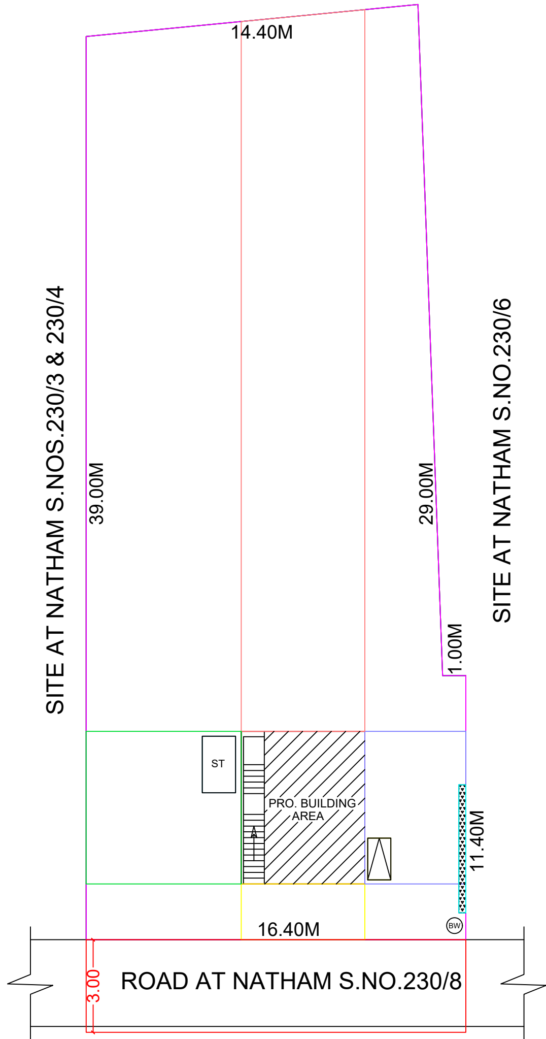
SITE PLAN
