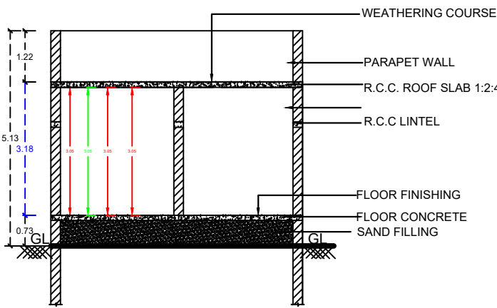
SECTION A1-A1
