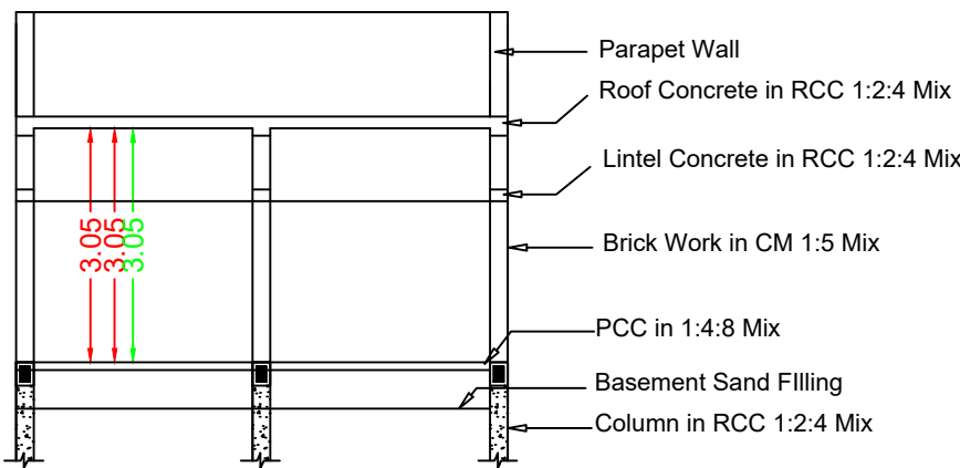
Section RR
