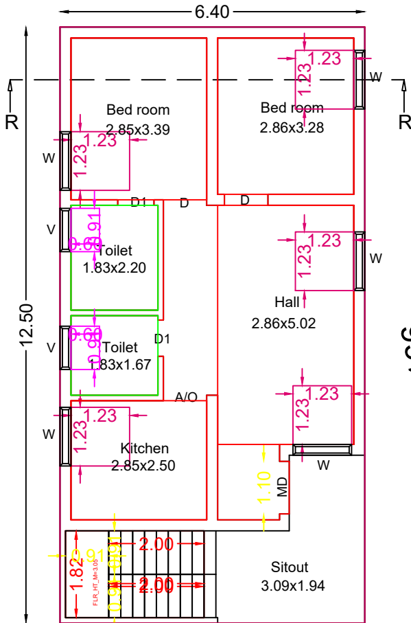
Pro.Ground Floor Plan
