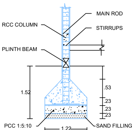
COLUMN DETAILS
