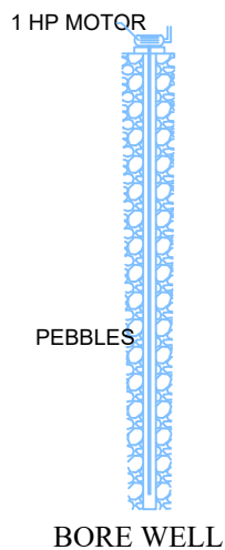
BORE WELL
