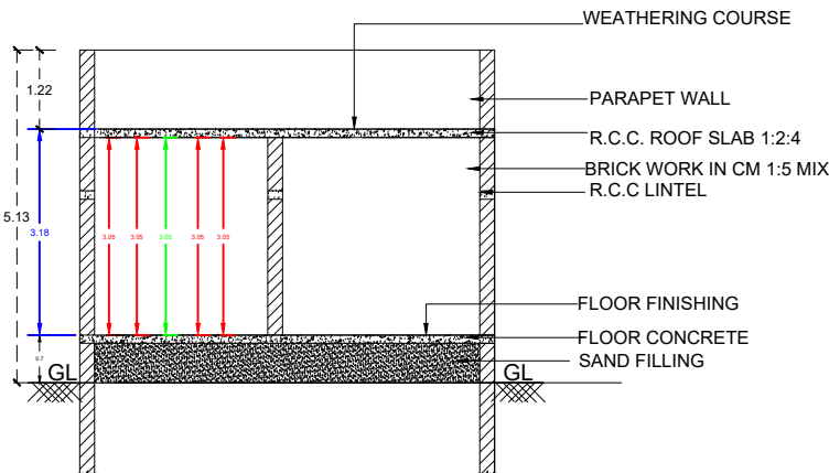
SECTION A1-A1
