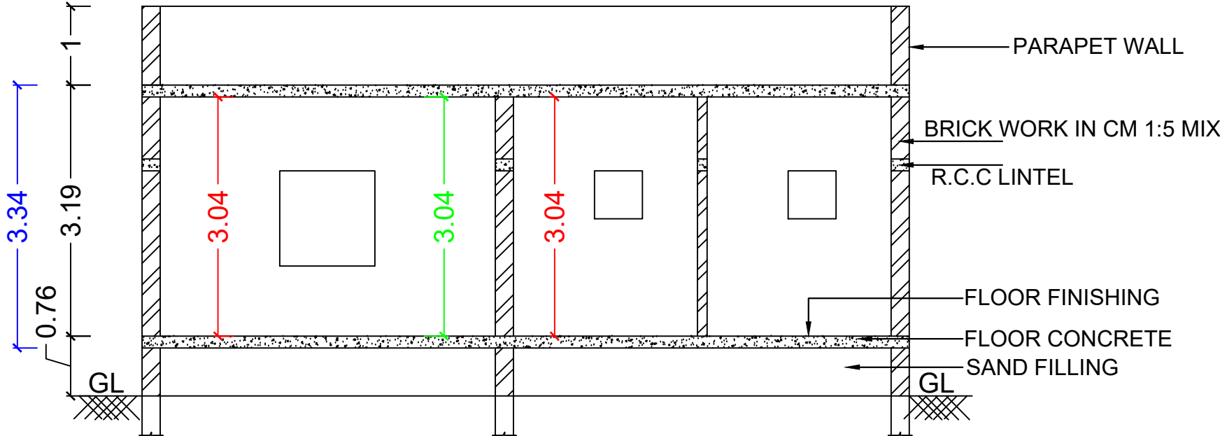
SECTION AT A1-A1
