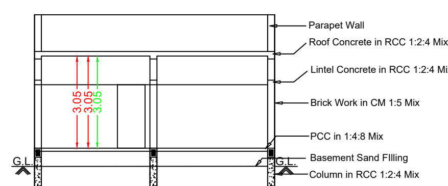
Section RR
