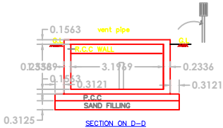
SECTION ON D-D
