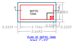
PLAN OF SEPTIC TANK
