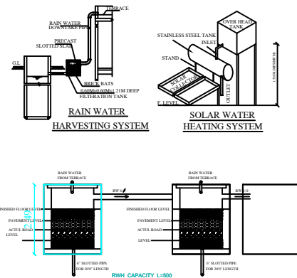
CUT SECTION ON AA
