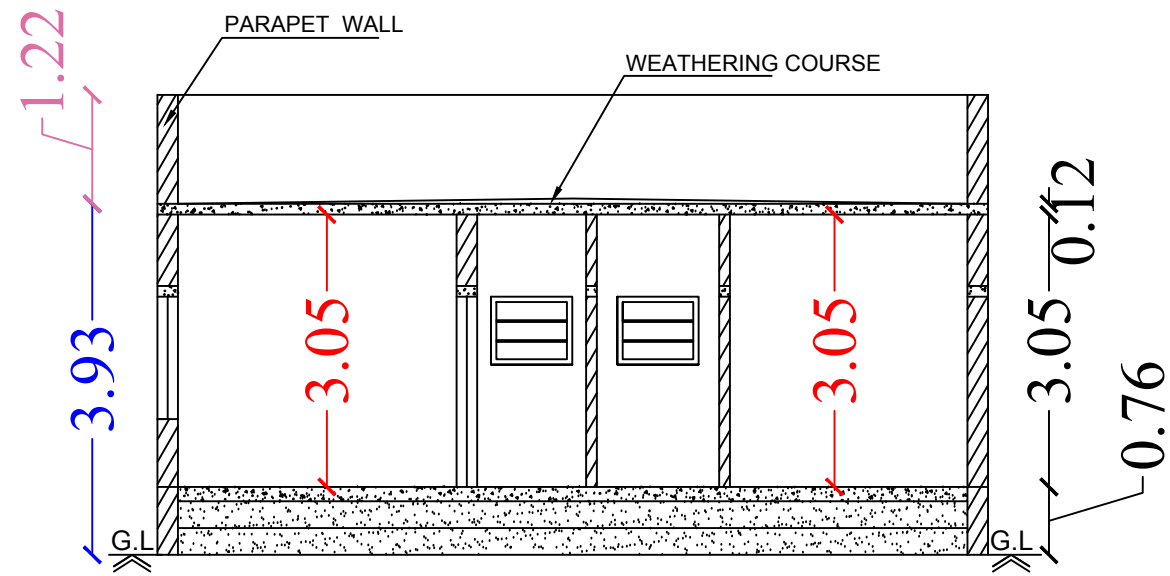
Section on-"AA"
