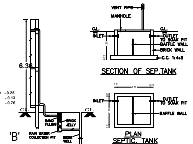
RAIN WATER HARVESTING SYSTEM RWH_CAPACITY_L=1000LTRS
