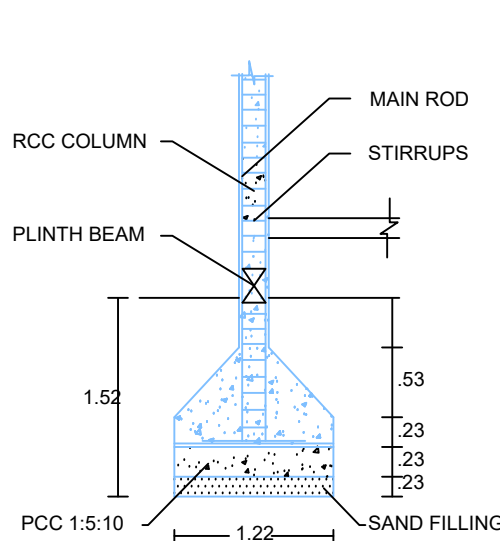
COLUMN DETAILS
