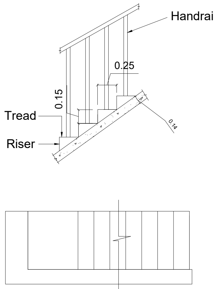
STAIRCASE DETAIL
