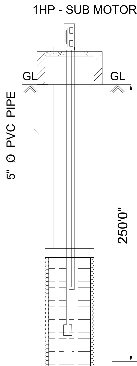
BOREWELL DETAILS
