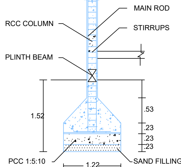
COLUMN DETAILS
