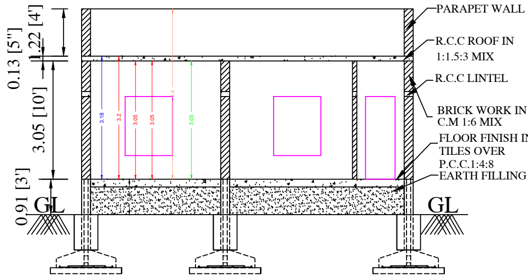
SECTION AA
