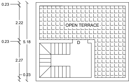
TERRACE FLOOR
