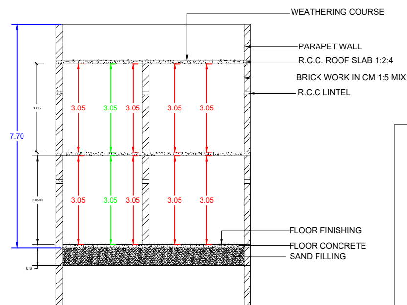
SECTION A1-A1
