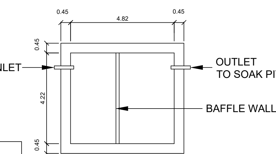
PLAN
