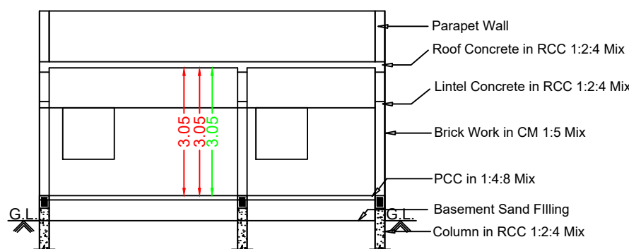
Section RR
