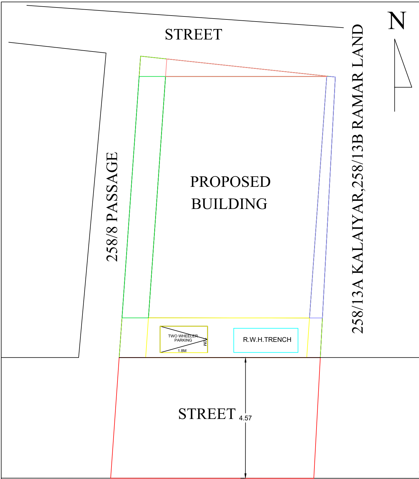
SITE PLAN
