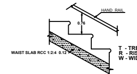
STAIR CASE DETAILS
