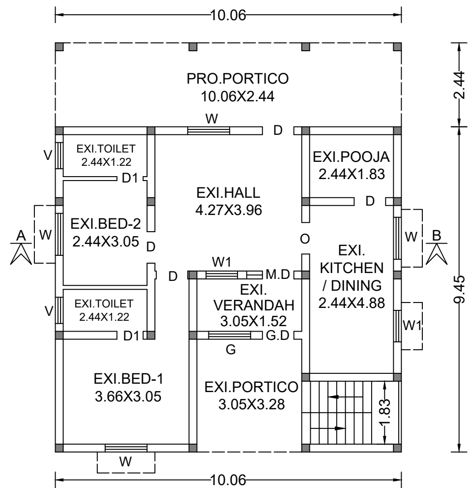
EXISTING AND PROPOSED GROUND FLOOR PLAN
