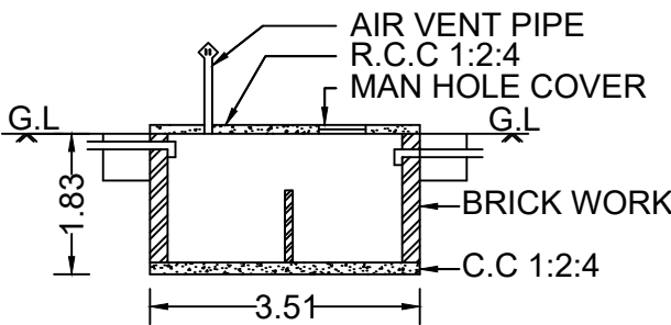
EXI.SEPTICTANK DETAILS
