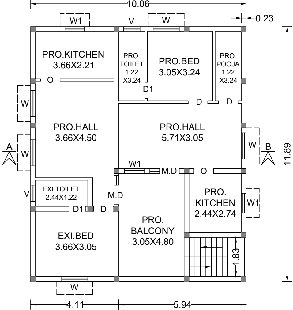
EXISTING AND PROPOSED FIRST FLOOR PLAN
