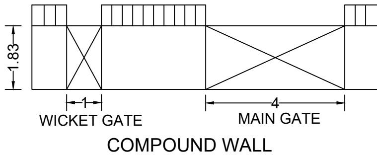
COMPOUND WALL
