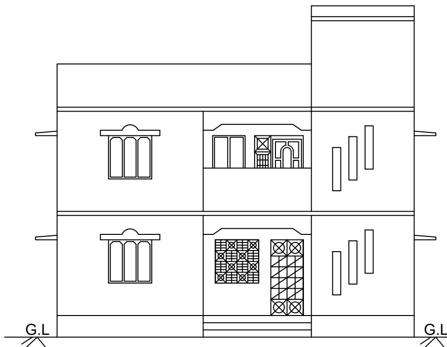
FRONT ELEVATION
