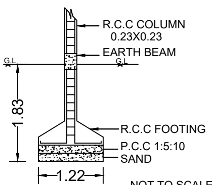
EXI.FOUNDATION DETAILS
