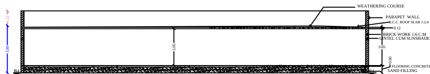
Section on-"AA"
