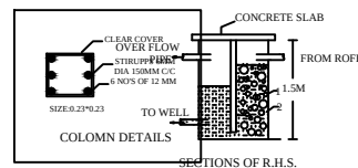
SECTIONS OF R.H.S.
