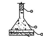
1.SAND FILLING FOR FOUNDATION 2.FOUNDATION CONCRETE P.C.C 1:5:10 3.RCC COLUMN FOOTING 4.PLINTHBEAM FOUNDATION DETAILS
