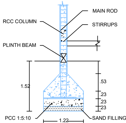
COLUMN DETAILS
